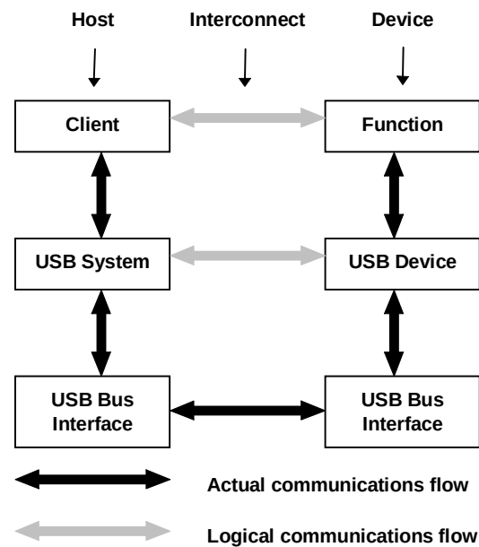
Figure 10-1. Interlayer Communications Model
