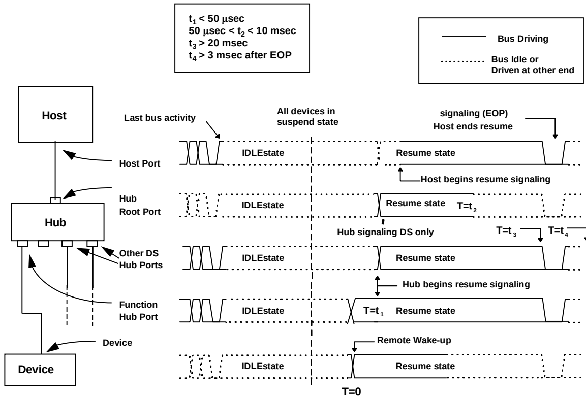
Figure 11-12. Resume Signaling
