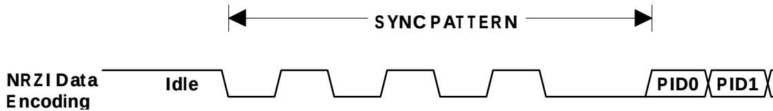
Figure 7-15. Sync Pattern
